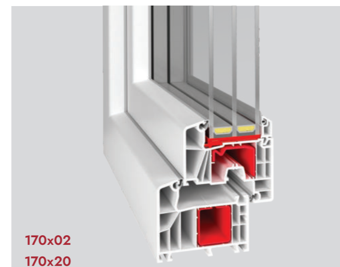
IDEAL 7000
